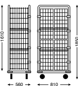
> TRANSLINGE TROLLEY ref: 9 940 20 50 4 independent doors. 3 melamine-coated shelves 2 of which can be raised. Capacity: 490 dm 3 . Weight: 60 kg. 4 casters ø 125 mm, 2 fixed and 2 swivelling.
